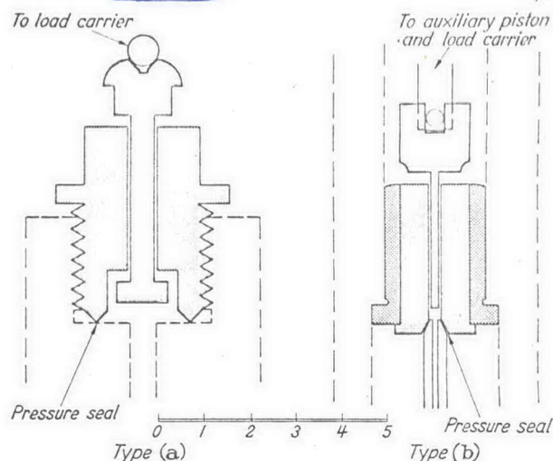
Fig. 2. Diagrams of piston-cylinder assemblies (Scale of cm)
